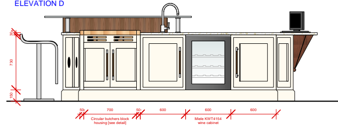
ELEVATION D
