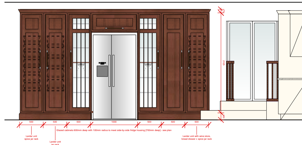
ELEVATION C
